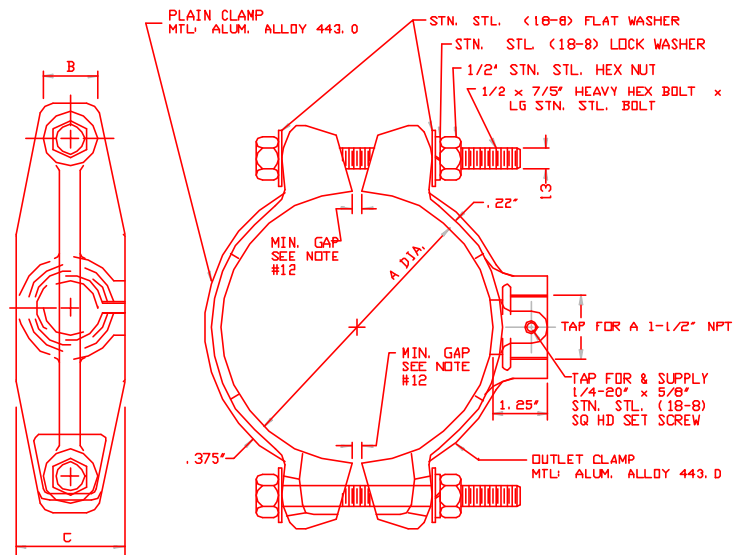
POLE CLAMP ASSEMBLY PEDESTRIAN CLAMP TYPE NTS
