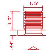
1-1/2" CHASE NIPPLE MTL: BRZ. 85-5-5-5 NTS
