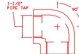
ELBOW MTL: ALUM. ALLOY 443.0
