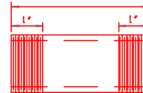
STD. 1-1/2" NIPPLE MTL: ALUM ALLOY 6061-T6 ASTM B-241
