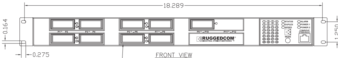
FRONT VIEW
