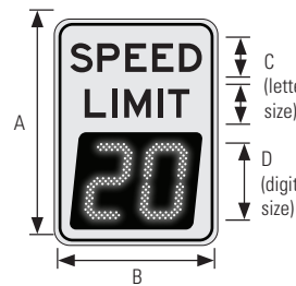
R2-1 Speed Limit Sign
