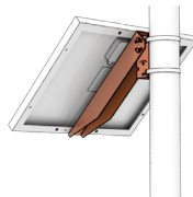
Side of Pole Mount
