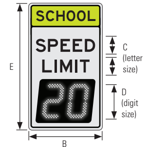
S5-1 School Zone Speed Limit Sign (15-inch model only)
